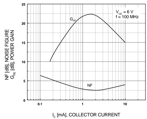
Figure 17. Power Gain & NF
